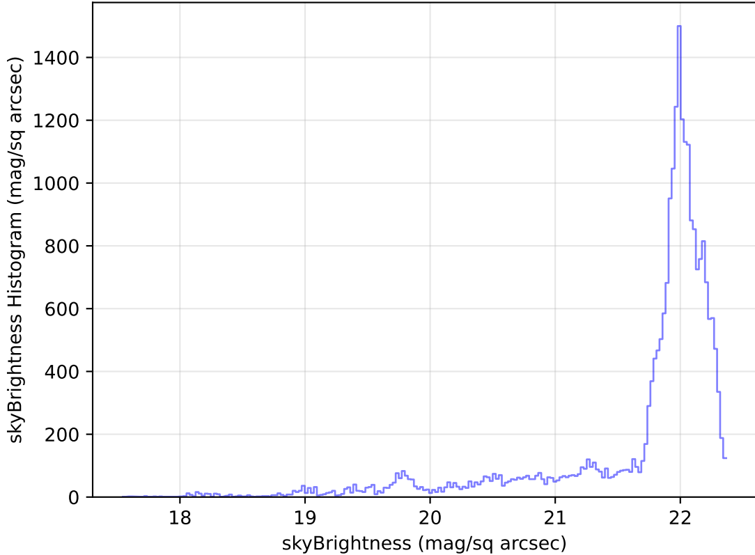
too_elab_heavy_r32_d3_ugrizy_v3.4_10yrs Yr 1 g band: skyBrightness Histogram
