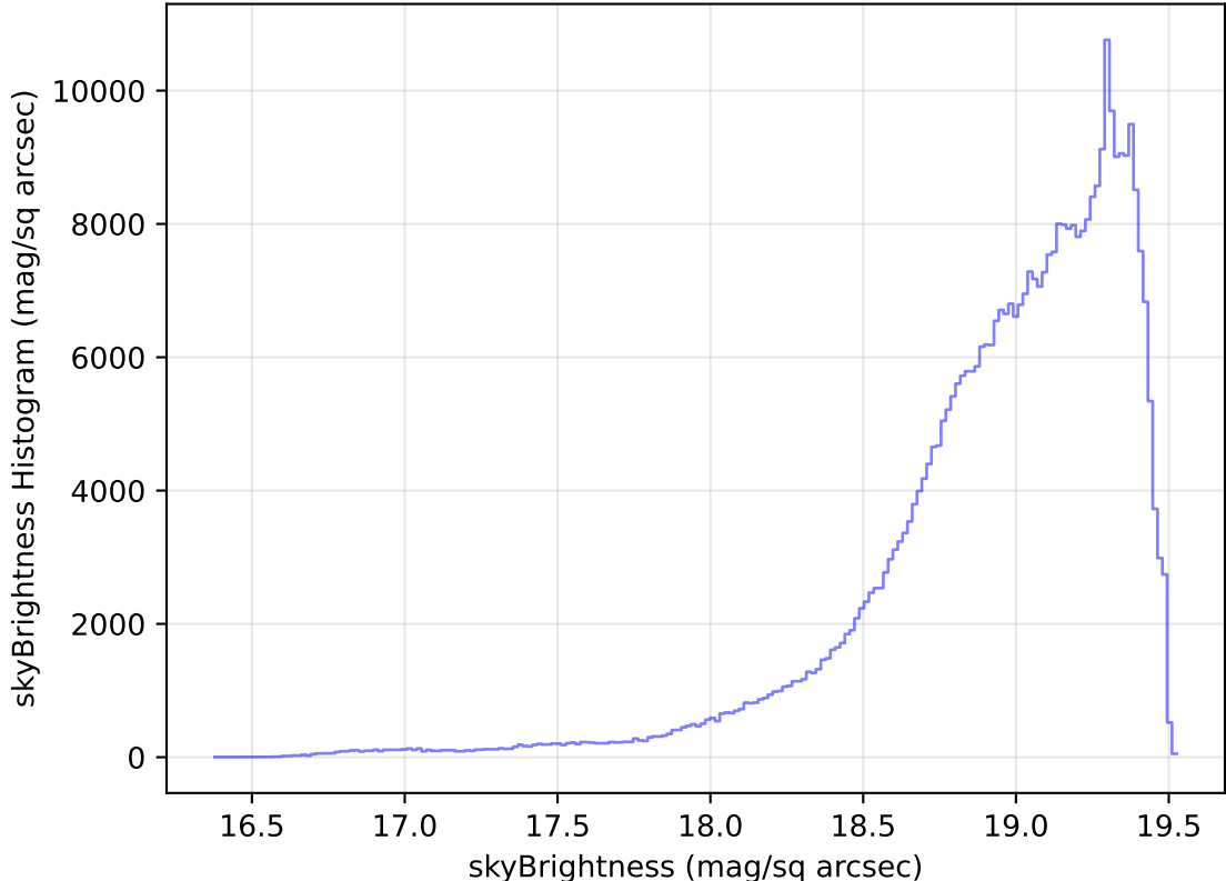
too_elab_heavy_r32_d3_ugrizy_v3.4_10yrs WFD z band: skyBrightness Histogram
