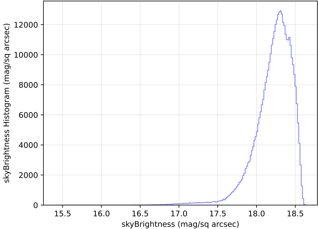
too_elab_heavy_r32_d3_ugrizy_v3.4_10yrs WFD y band: skyBrightness Histogram
