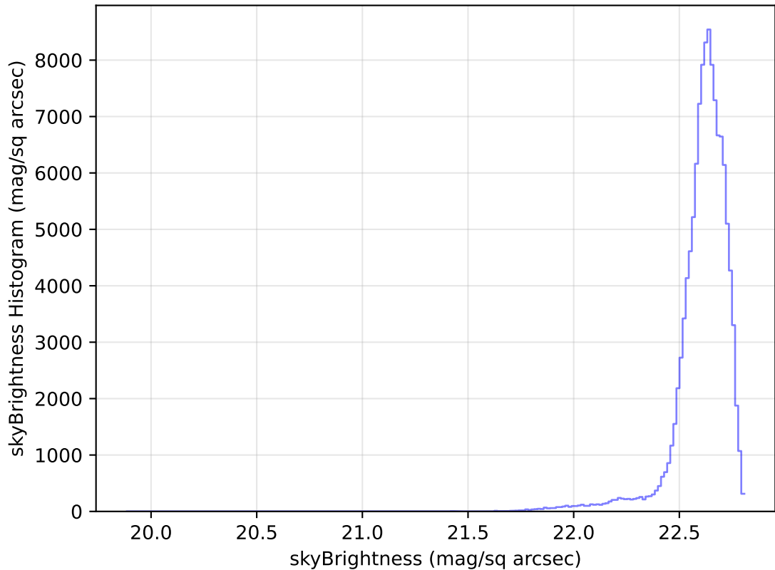
too_elab_heavy_r32_d3_ugrizy_v3.4_10yrs WFD u band: skyBrightness Histogram
