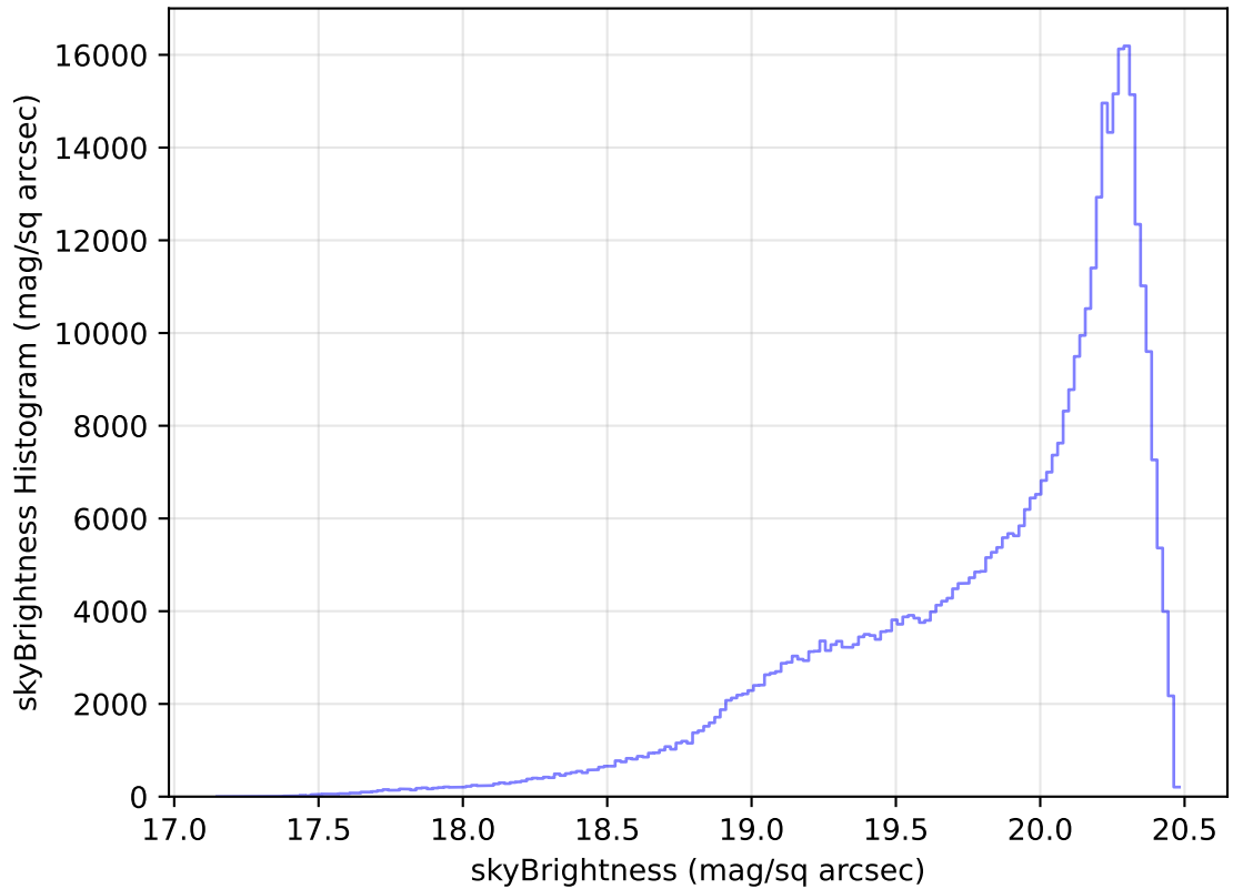
too_elab_heavy_r32_d3_ugrizy_v3.4_10yrs WFD i band: skyBrightness Histogram
