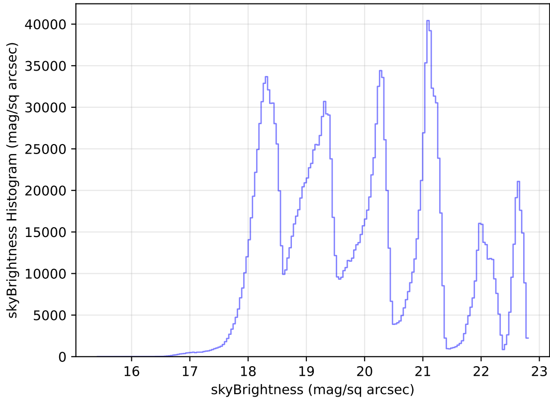
too_elab_heavy_r32_d3_ugrizy_v3.4_10yrs WFD all bands: skyBrightness Histogram
