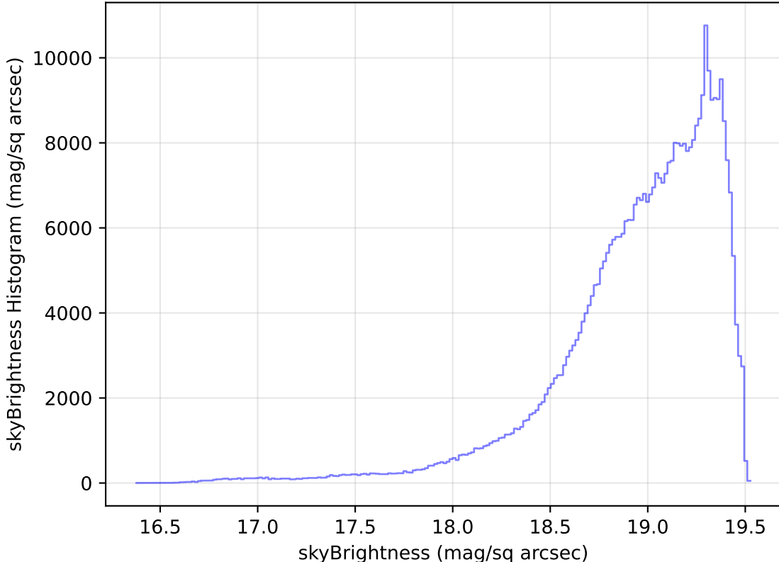
too_elab_heavy_r32_d3_ugrizy_v3.4_10yrs All sky z band: skyBrightness Histogram
