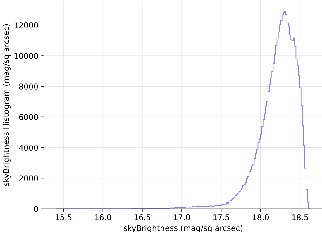
too_elab_heavy_r32_d3_ugrizy_v3.4_10yrs All sky y band: skyBrightness Histogram
