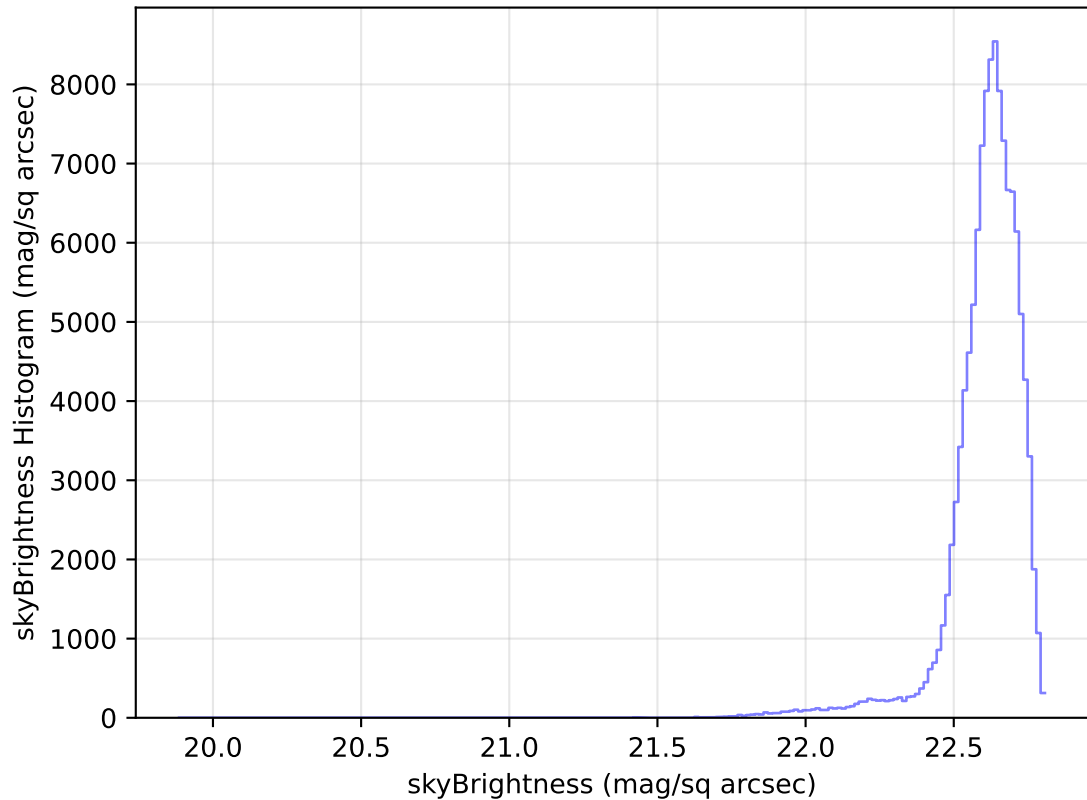
too_elab_heavy_r32_d3_ugrizy_v3.4_10yrs All sky u band: skyBrightness Histogram
