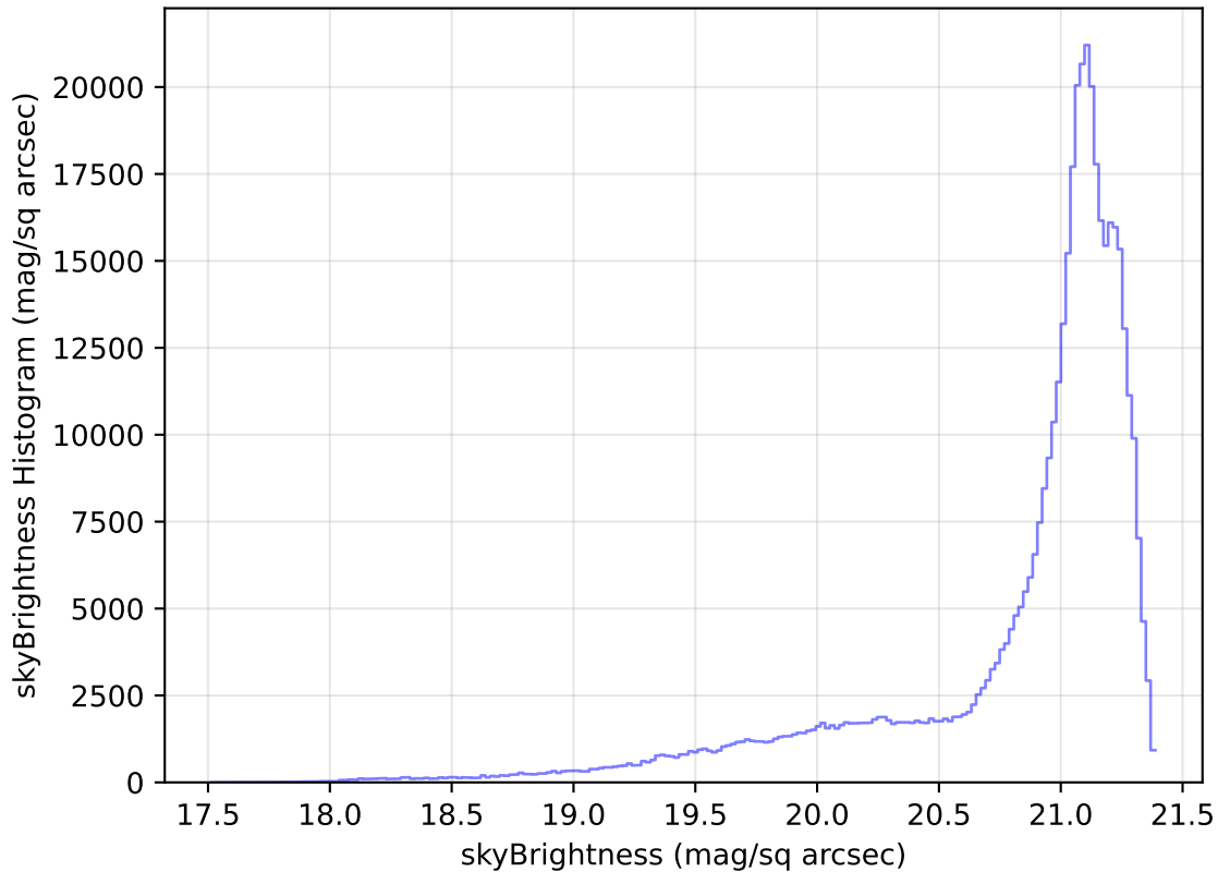
too_elab_heavy_r32_d3_ugrizy_v3.4_10yrs All sky r band: skyBrightness Histogram
