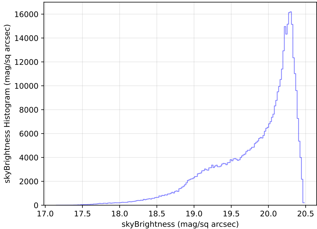
too_elab_heavy_r32_d3_ugrizy_v3.4_10yrs All sky i band: skyBrightness Histogram
