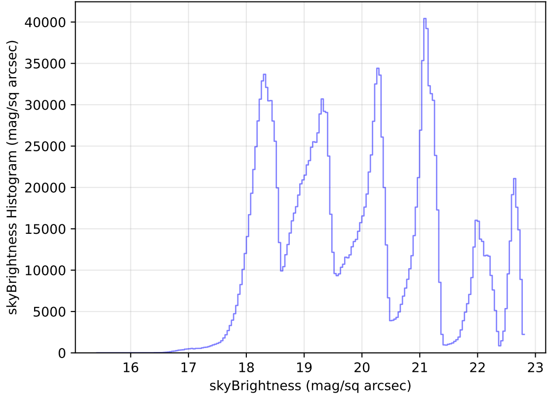
too_elab_heavy_r32_d3_ugrizy_v3.4_10yrs All sky all bands: skyBrightness Histogram
