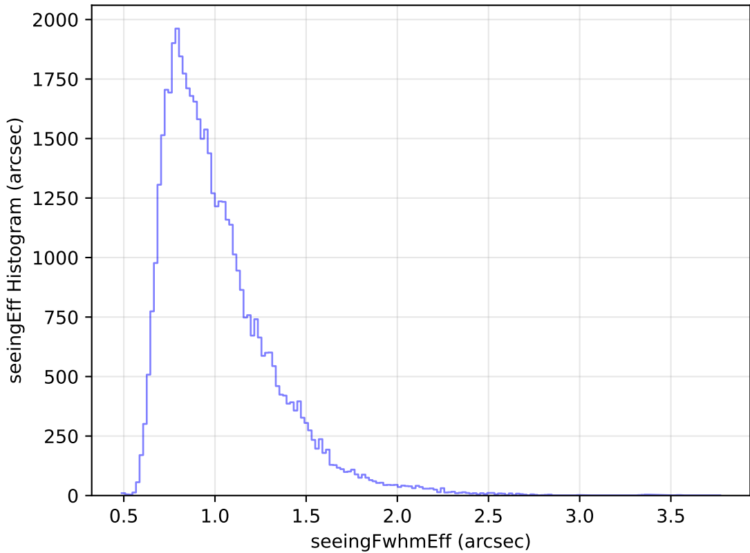
too_elab_heavy_r32_d3_ugrizy_v3.4_10yrs Yr 1 r band: seeingEff Histogram
