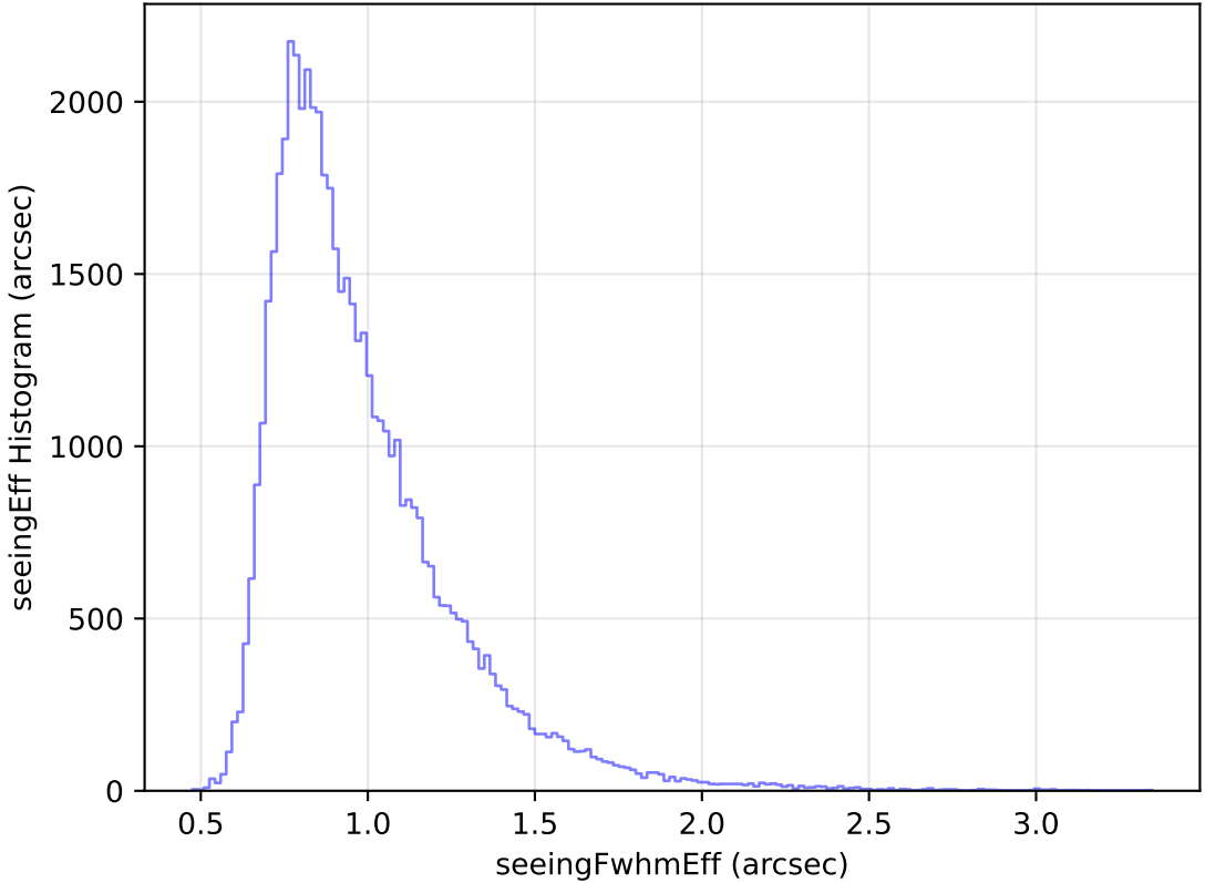
too_elab_heavy_r32_d3_ugrizy_v3.4_10yrs Yr 1 i band: seeingEff Histogram
