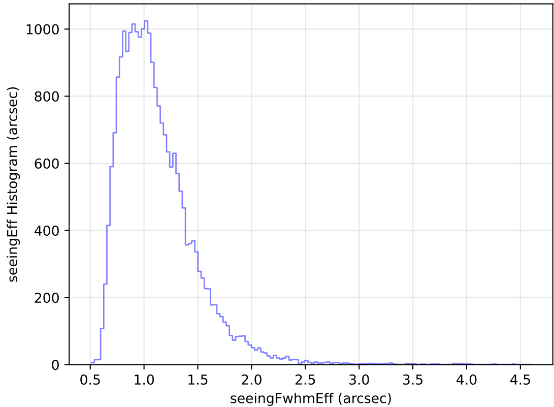
too_elab_heavy_r32_d3_ugrizy_v3.4_10yrs Yr 1 g band: seeingEff Histogram
