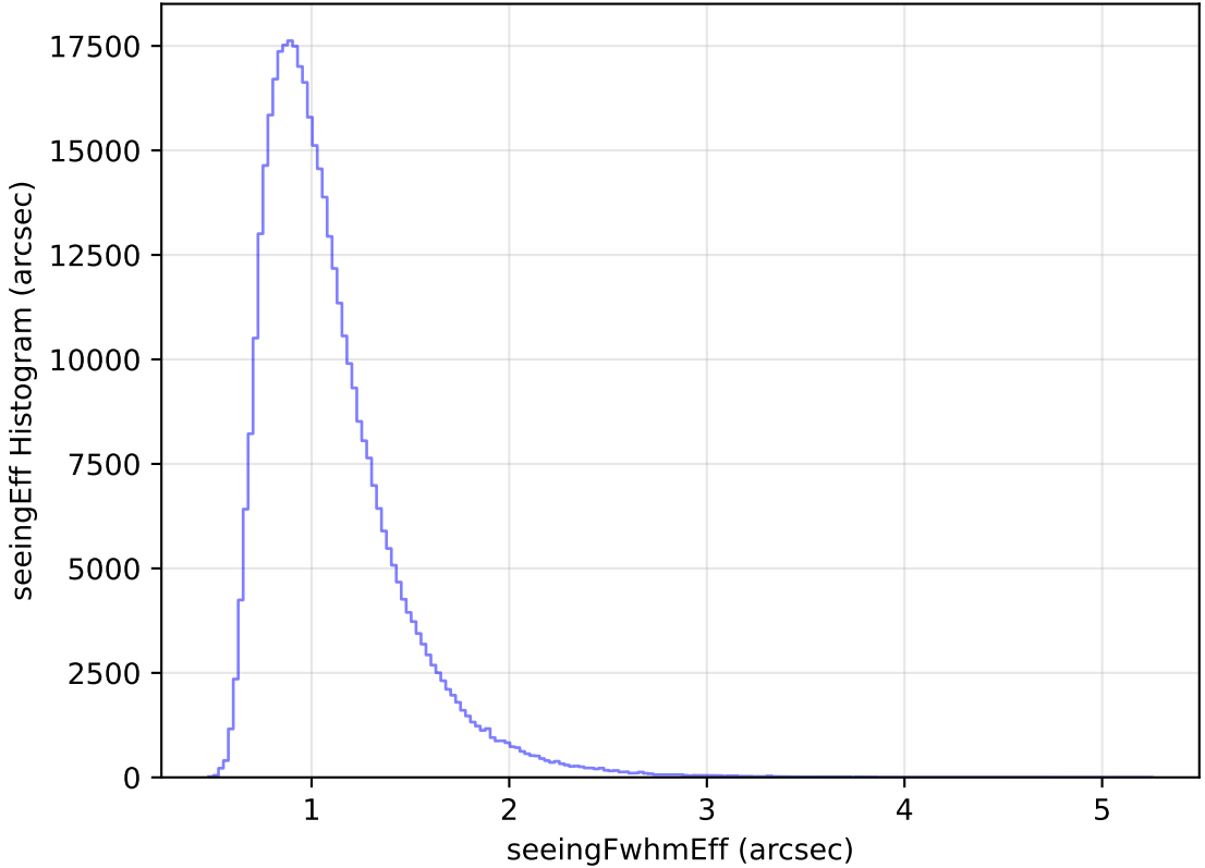
too_elab_heavy_r32_d3_ugrizy_v3.4_10yrs WFD z band: seeingEff Histogram
