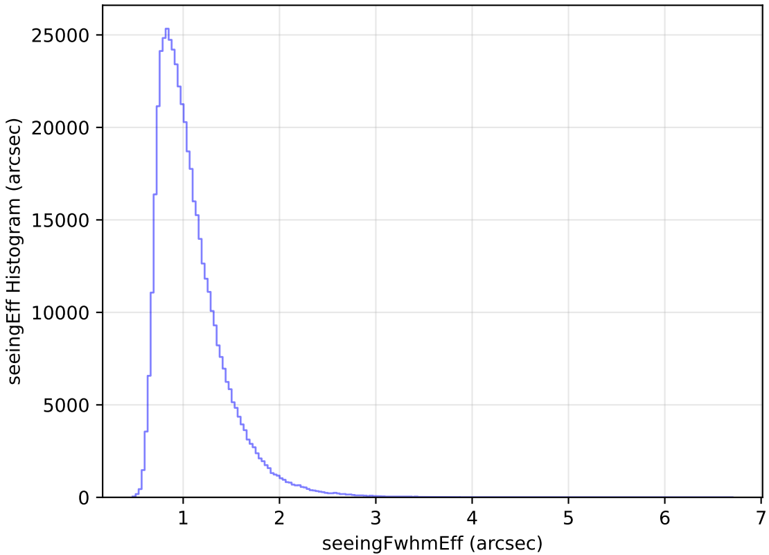
too_elab_heavy_r32_d3_ugrizy_v3.4_10yrs WFD i band: seeingEff Histogram
