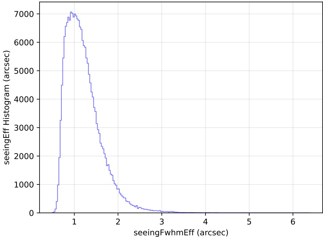
too_elab_heavy_r32_d3_ugrizy_v3.4_10yrs WFD g band: seeingEff Histogram
