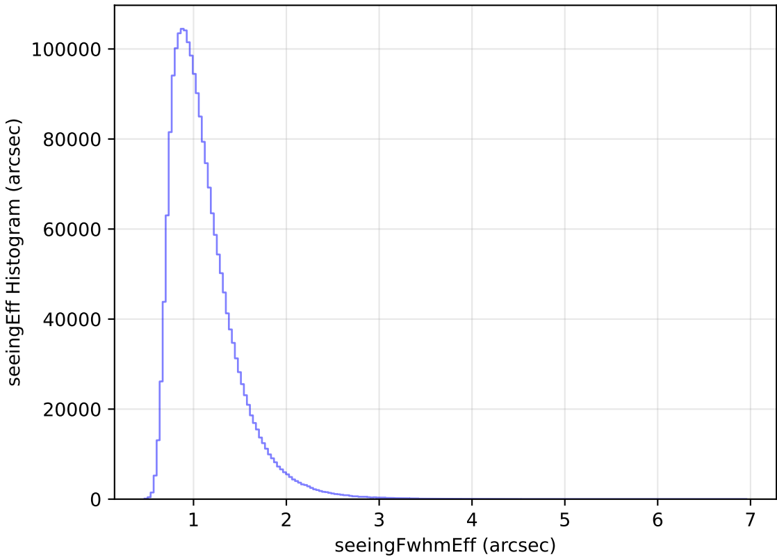
too_elab_heavy_r32_d3_ugrizy_v3.4_10yrs WFD all bands: seeingEff Histogram
