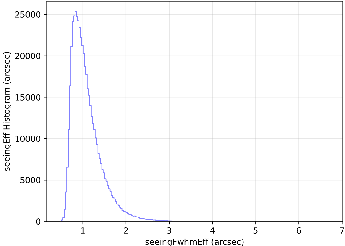
too_elab_heavy_r32_d3_uigrzy_v3.4_10yrs All sky i band: seeingEff Histogram
