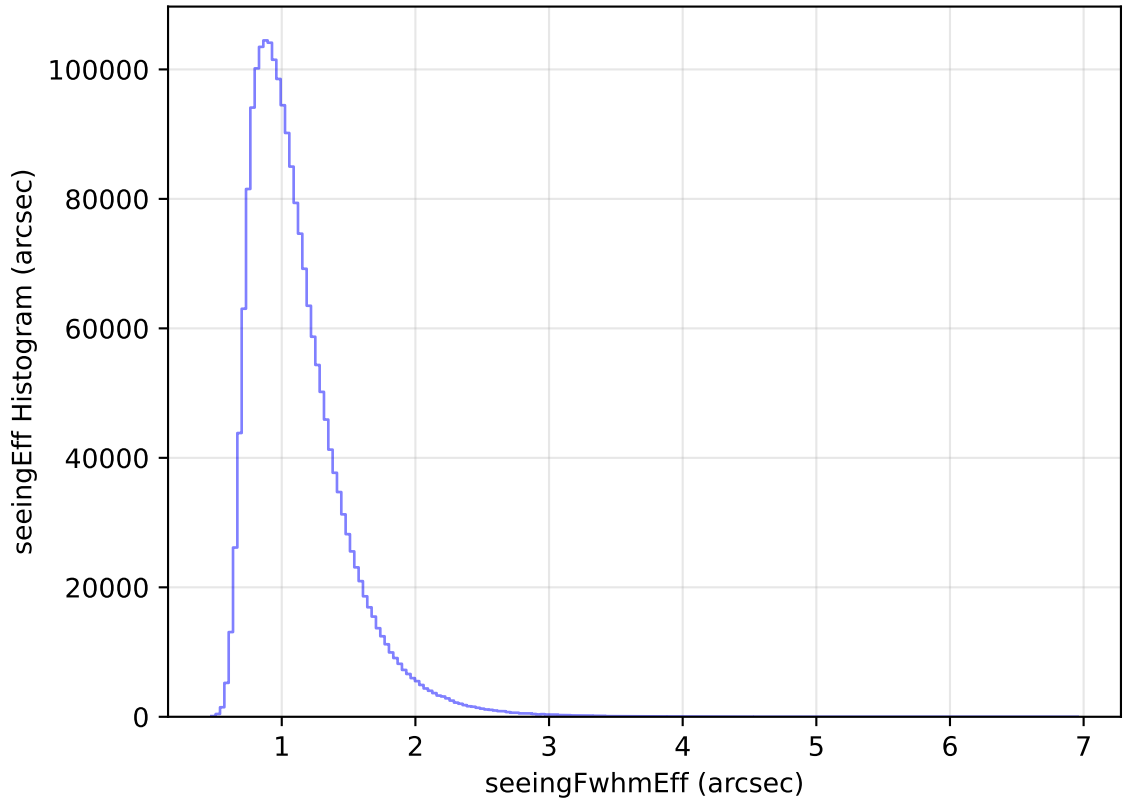
too_elab_heavy_r32_d3_uigrizy_v3.4_10yrs All sky all bands: seeingEff Histogram
