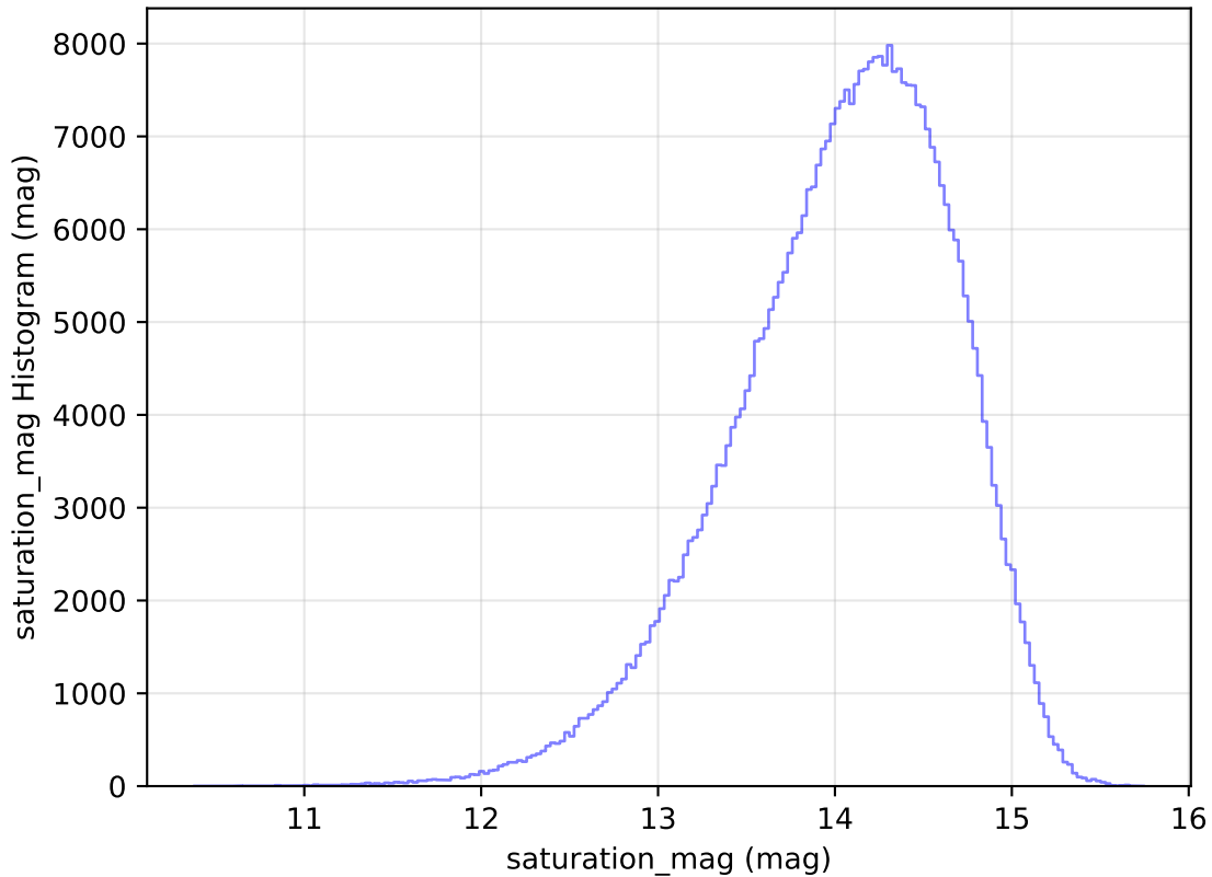
too_elab_heavy_r32_d3_ugrizy_v3.4_10yrs WFD z band: saturation_mag Histogram
