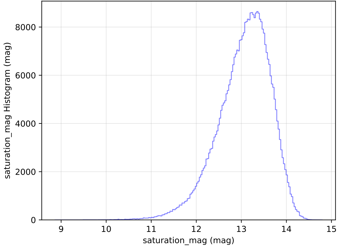
too_elab_heavy_r32_d3_ugrizy_v3.4_10yrs WFD y band: saturation_mag Histogram
