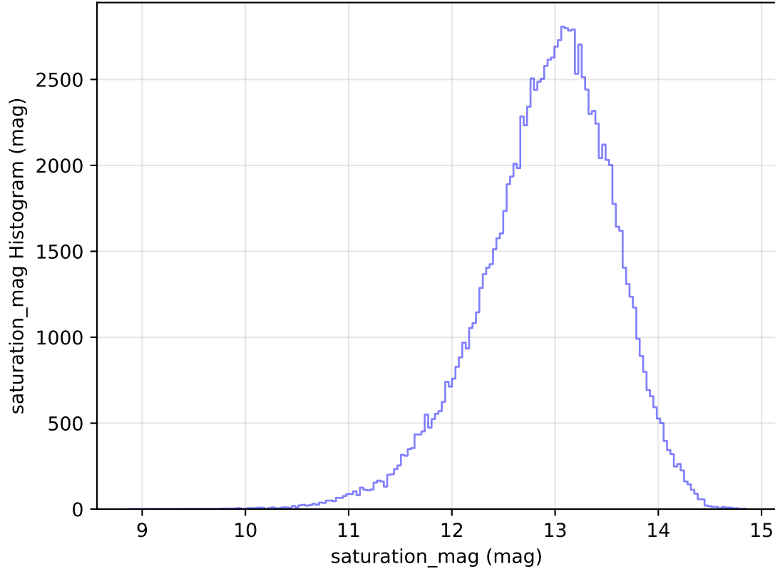
too_elab_heavy_r32_d3_ugrizy_v3.4_10yrs WFD u band: saturation_mag Histogram
