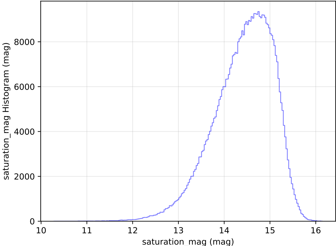
too_elab_heavy_r32_d3_ugrizy_v3.4_10yrs WFD i band: saturation_mag Histogram
