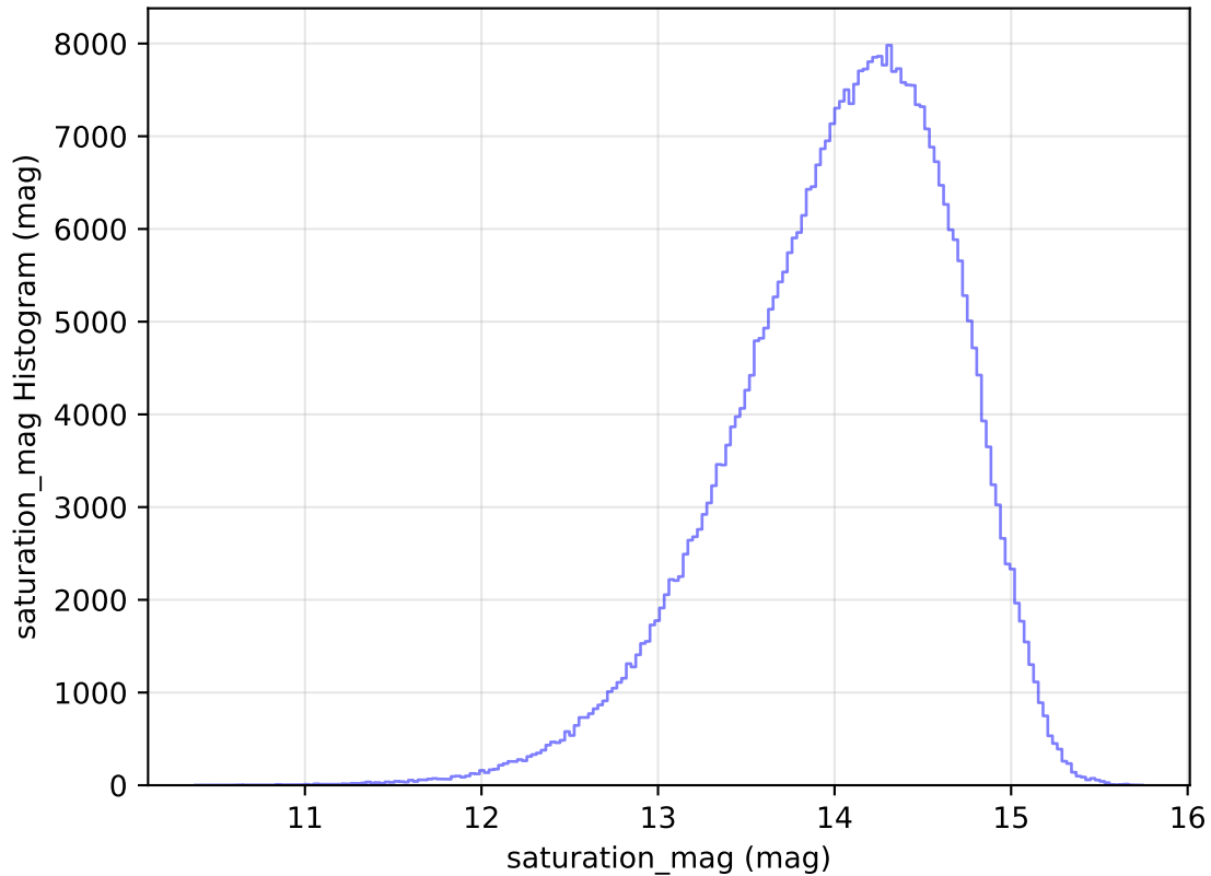
too_elab_heavy_r32_d3_ugrizy_v3.4_10yrs All sky z band: saturation_mag Histogram
