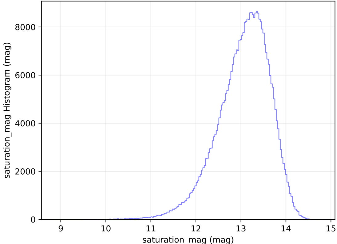
too_elab_heavy_r32_d3_ugrizy_v3.4_10yrs All sky y band: saturation_mag Histogram
