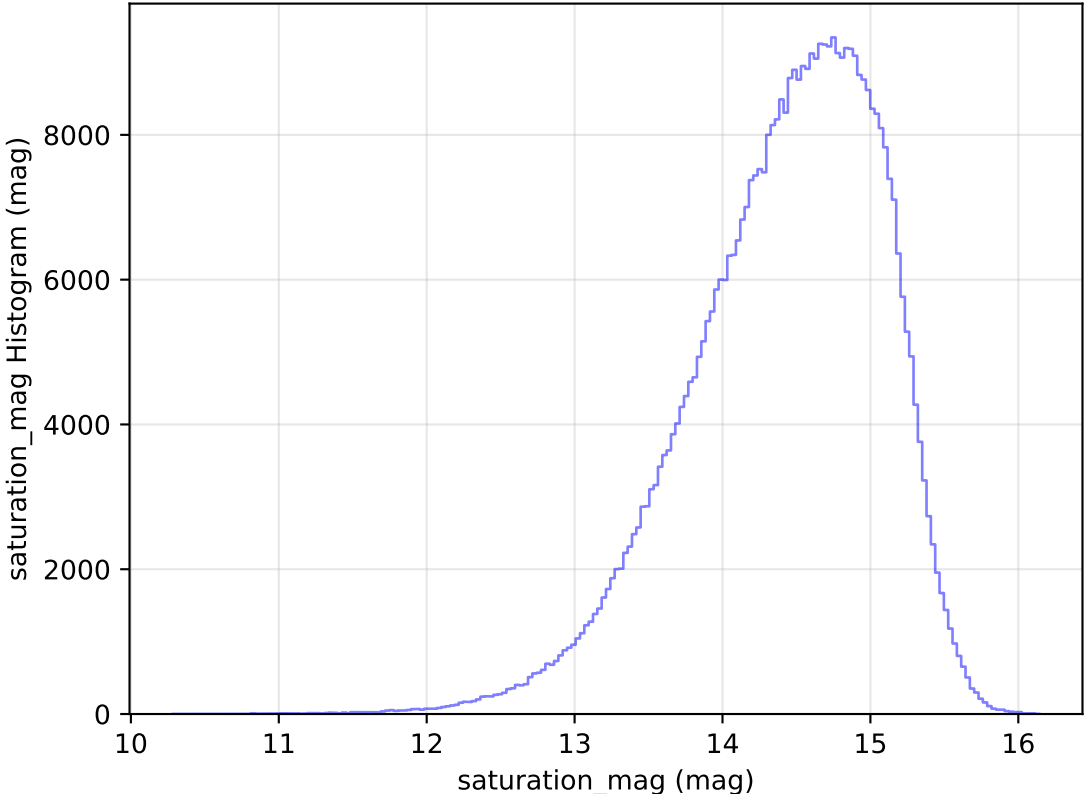
too_elab_heavy_r32_d3_ugrizy_v3.4_10yrs All sky i band: saturation_mag Histogram
