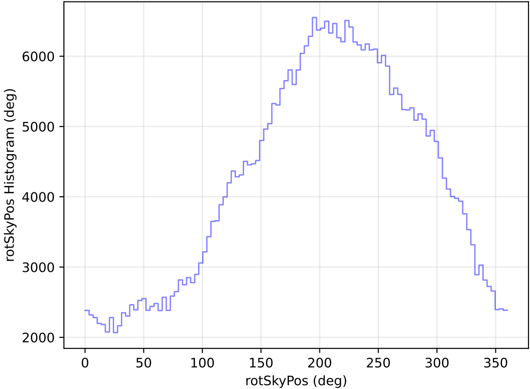
too_elab_heavy_r32_d3_ugrizy_v3.4_10yrs WFD z band: rotSkyPos Histogram
