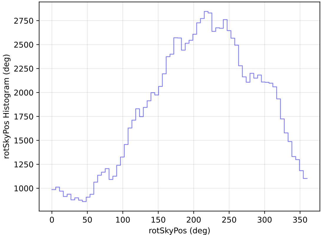
too_elab_heavy_r32_d3_ugrizy_v3.4_10yrs WFD u band: rotSkyPos Histogram
