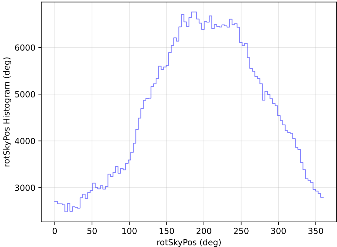
too_elab_heavy_r32_d3_ugrizy_v3.4_10yrs WFD r band: rotSkyPos Histogram
