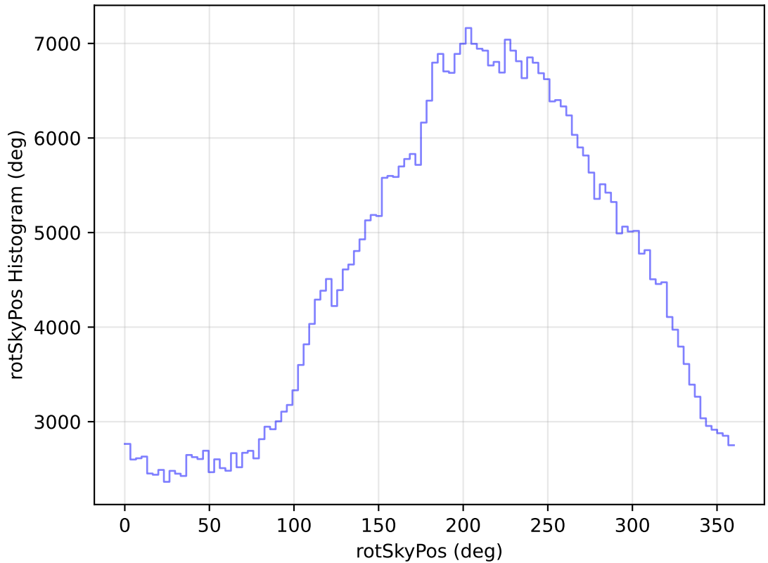
too_elab_heavy_r32_d3_ugrizy_v3.4_10yrs WFD i band: rotSkyPos Histogram
