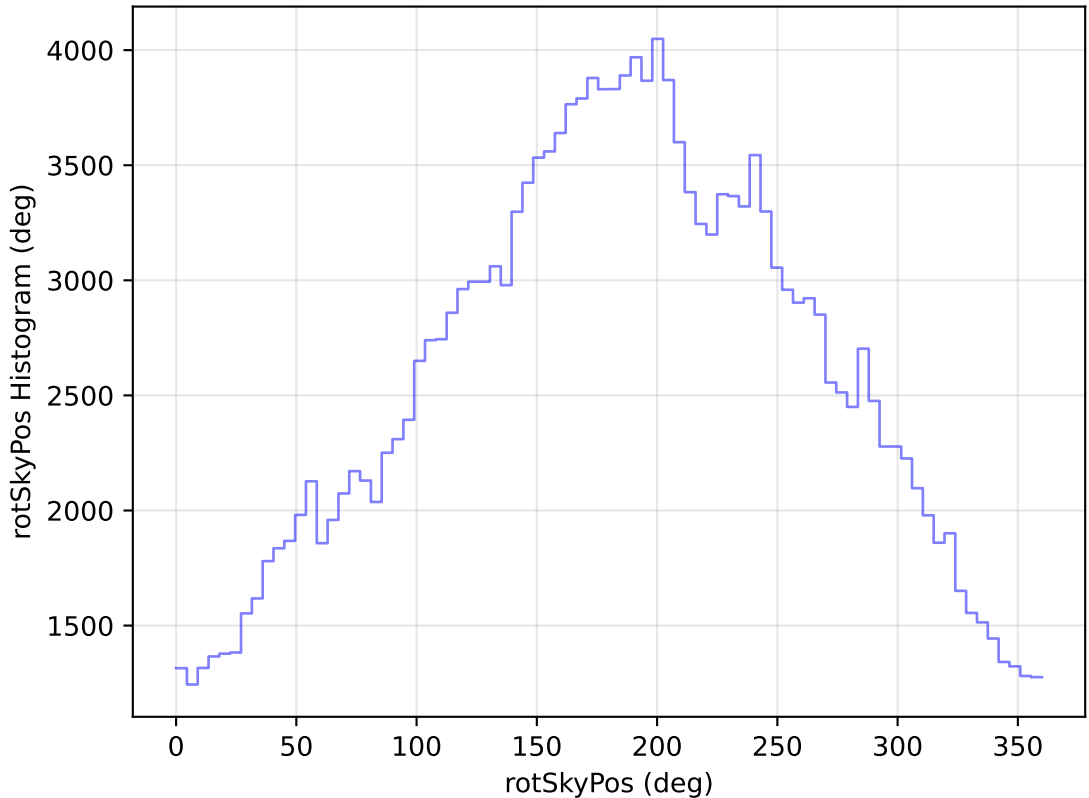
too_elab_heavy_r32_d3_ugrizy_v3.4_10yrs WFD g band: rotSkyPos Histogram
