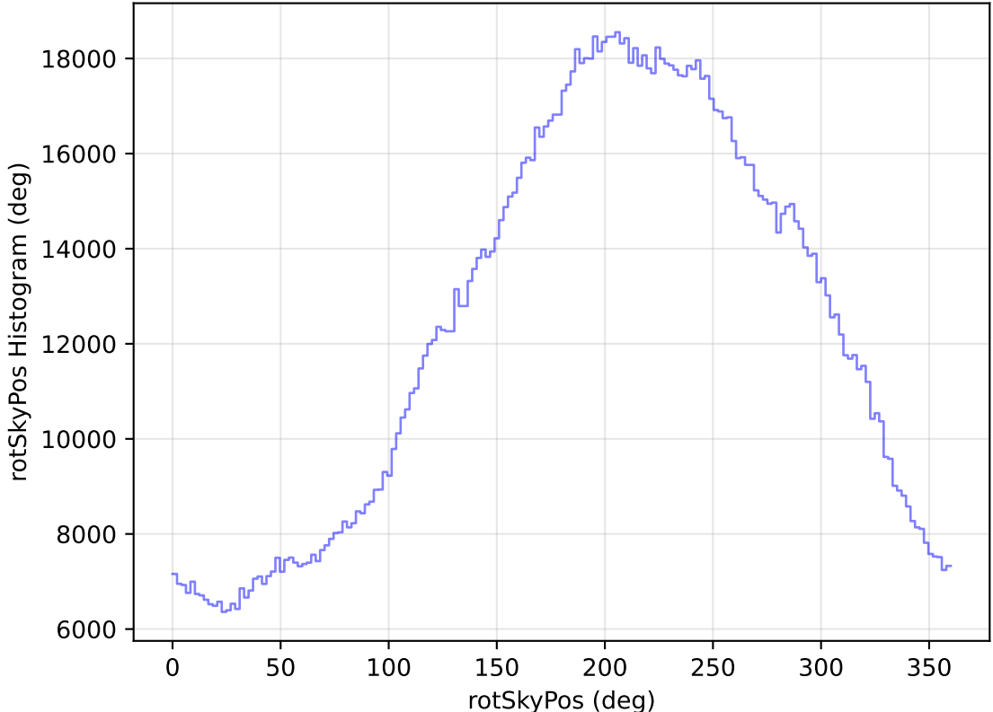
too_elab_heavy_r32_d3_ugrizy_v3.4_10yrs WFD all bands: rotSkyPos Histogram
