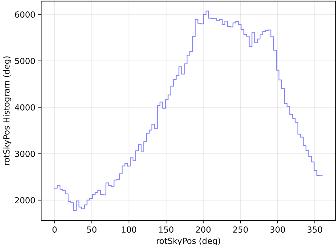
too_elab_heavy_r32_d3_ugrizy_v3.4_10yrs All sky y band: rotSkyPos Histogram
