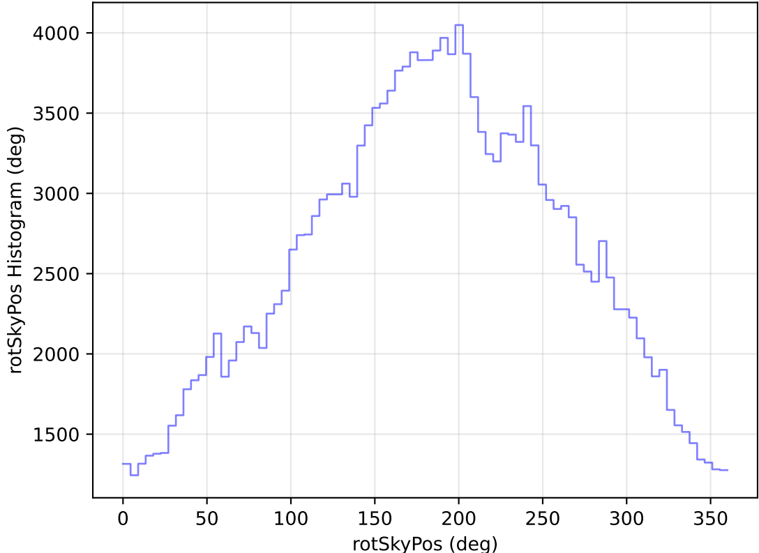
too_elab_heavy_r32_d3_ugrizy_v3.4_10yrs All sky g band: rotSkyPos Histogram
