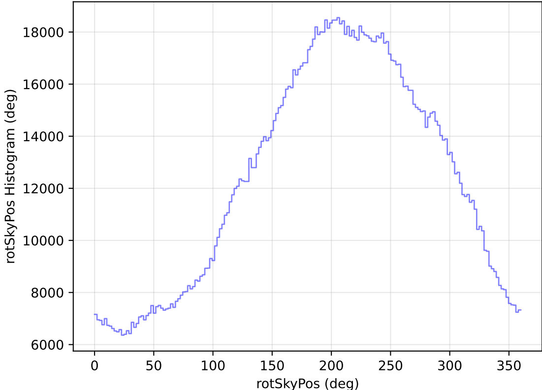
too_elab_heavy_r32_d3_ugrizy_v3.4_10yrs All sky all bands: rotSkyPos Histogram
