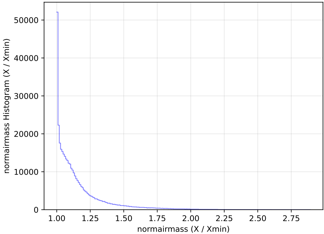
too_elab_heavy_r32_d3_ugrizy_v3.4_10yrs WFD y band: normairmass Histogram
