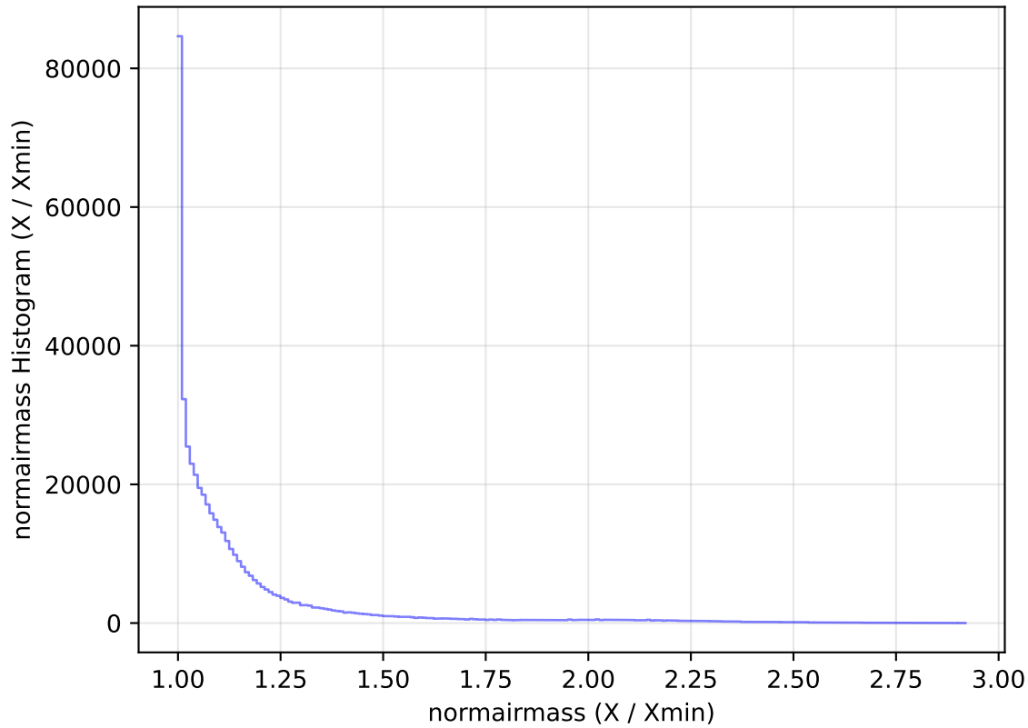
too_elab_heavy_r32_d3_ugrizy_v3.4_10yrs WFD i band: normairmass Histogram
