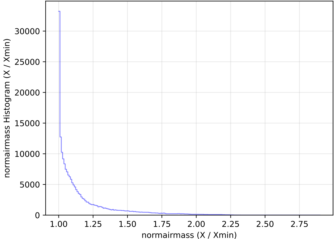
too_elab_heavy_r32_d3_ugrizy_v3.4_10yrs WFD g band: normairmass Histogram
