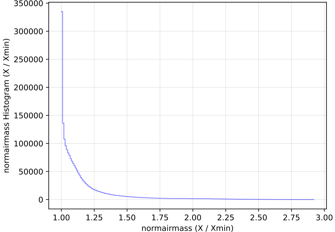
too_elab_heavy_r32_d3_ugrizy_v3.4_10yrs WFD all bands: normairmass Histogram
