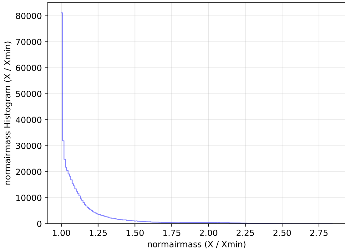
too_elab_heavy_r32_d3_ugrizy_v3.4_10yrs All sky r band: normairmass Histogram
