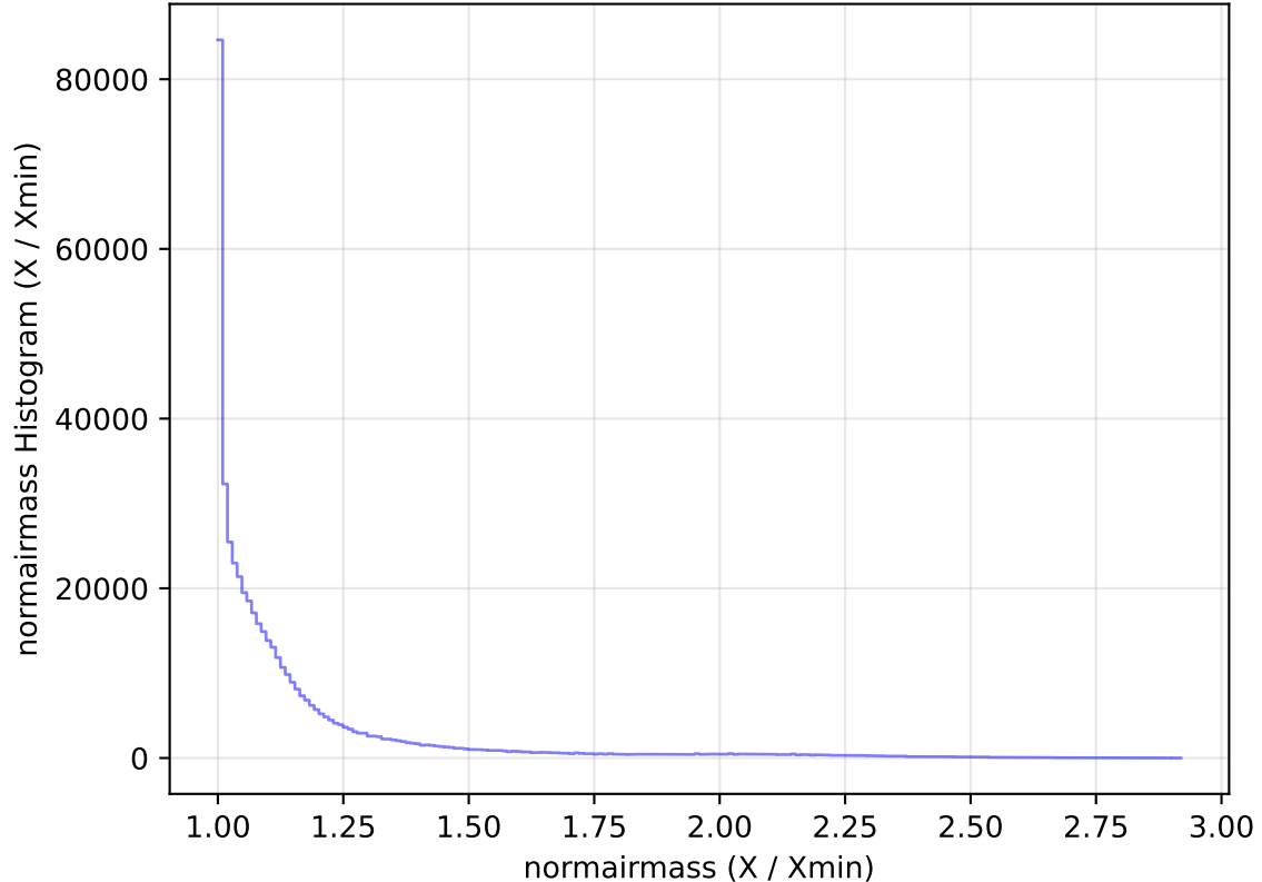
too_elab_heavy_r32_d3_ugrizy_v3.4_10yrs All sky i band: normairmass Histogram
