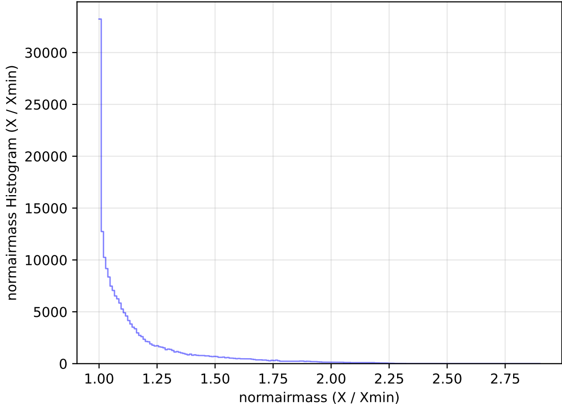
too_elab_heavy_r32_d3_ugrizy_v3.4_10yrs All sky g band: normairmass Histogram
