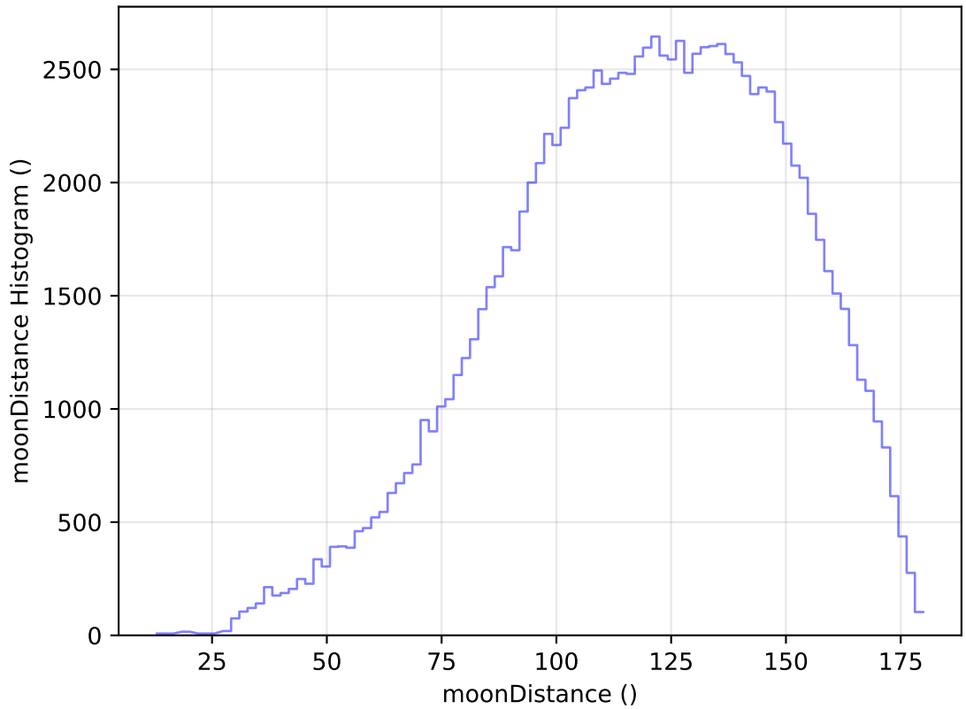
too_elab_heavy_r32_d3_ugrizy_v3.4_10yrs WFD u band: moonDistance Histogram
