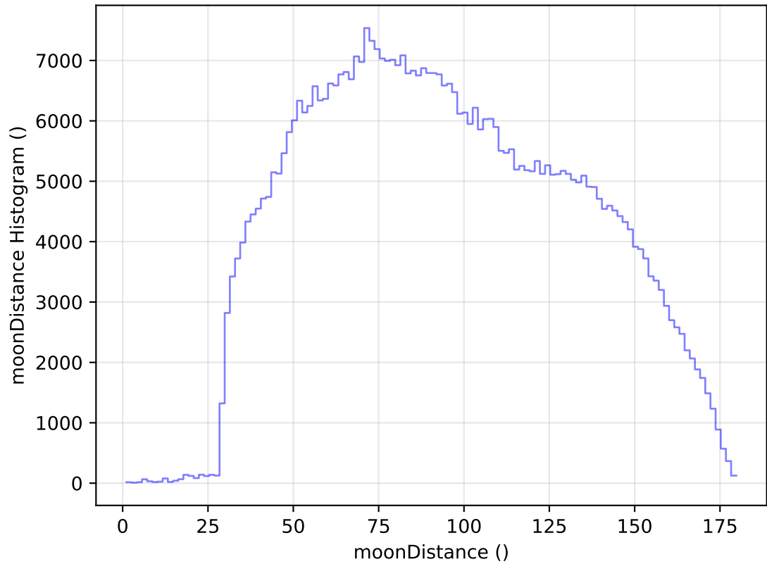
too_elab_heavy_r32_d3_ugrizy_v3.4_10yrs WFD i band: moonDistance Histogram
