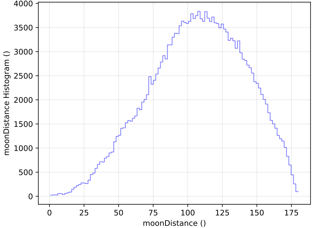
too_elab_heavy_r32_d3_ugrizy_v3.4_10yrs WFD g band: moonDistance Histogram
