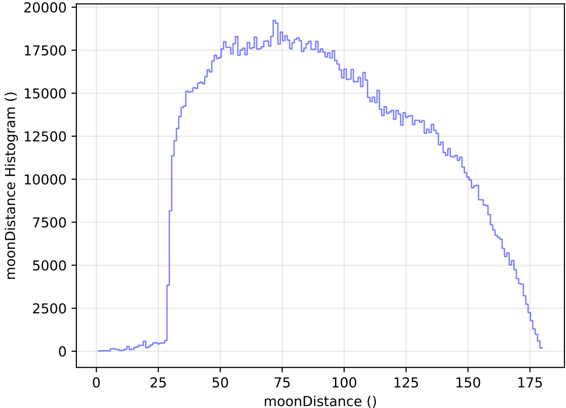
too_elab_heavy_r32_d3_ugrizy_v3.4_10yrs WFD all bands: moonDistance Histogram
