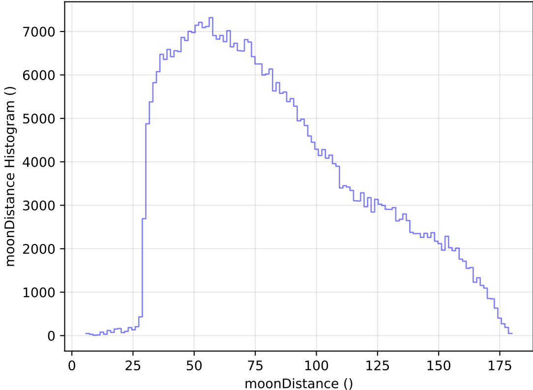
too_elab_heavy_r32_d3_ugrizy_v3.4_10yrs All sky z band: moonDistance Histogram
