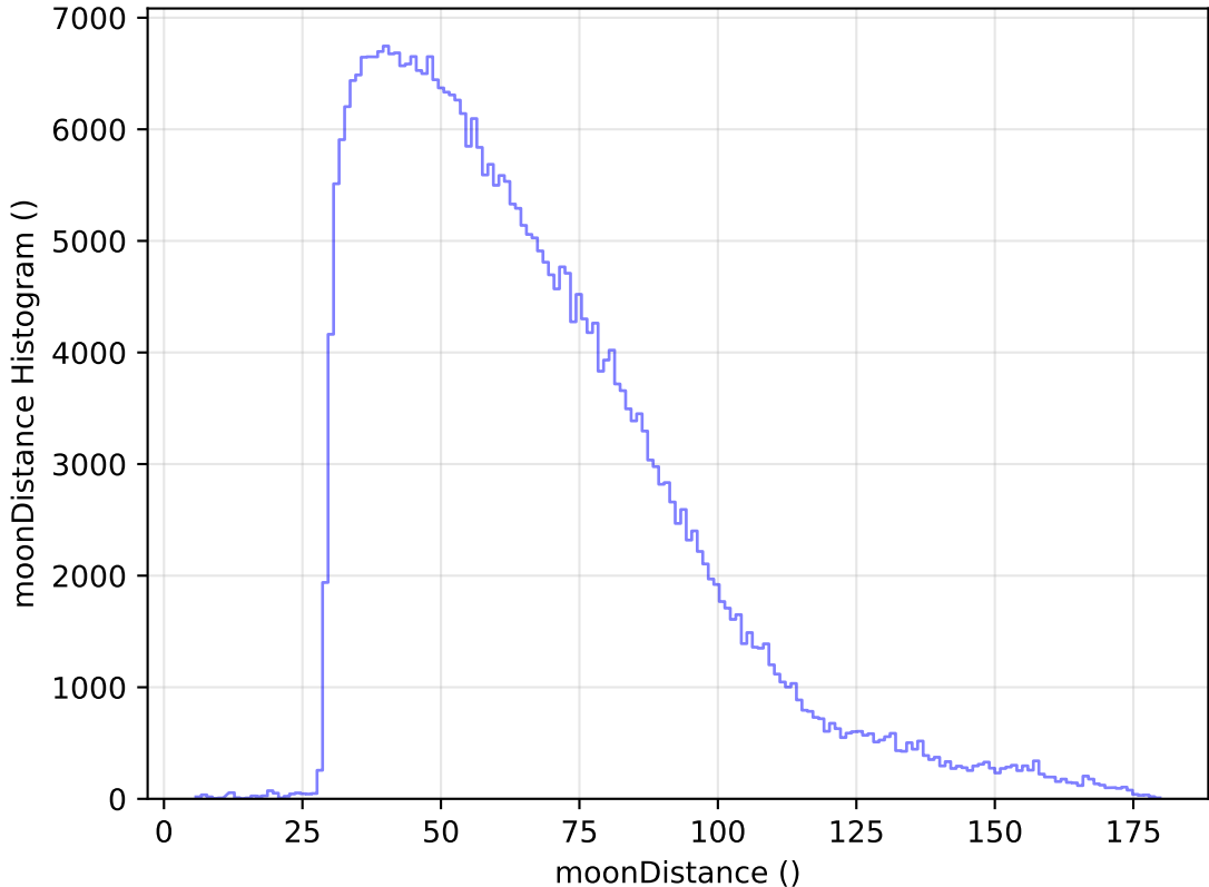
too_elab_heavy_r32_d3_ugrizy_v3.4_10yrs All sky y band: moonDistance Histogram
